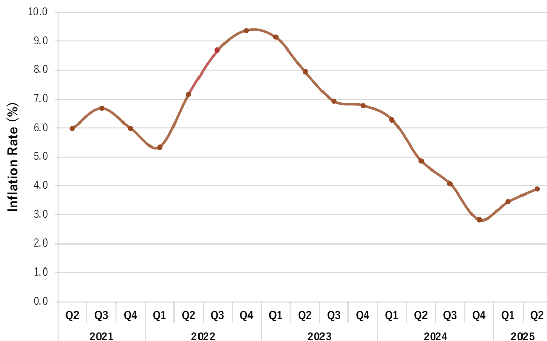
Figure 2: Inflation Rates, 2021-2025
