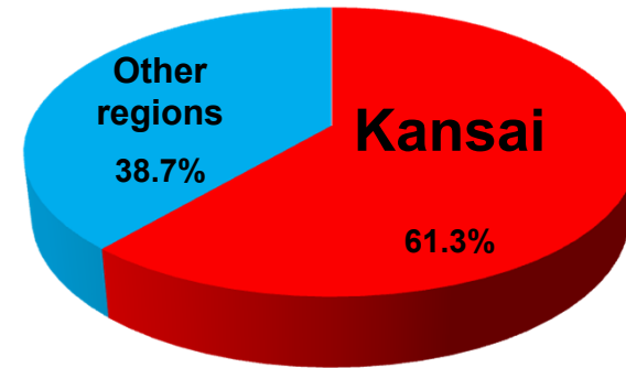
[Share of lithium-ion battery-related industries in Japan (2012)]
