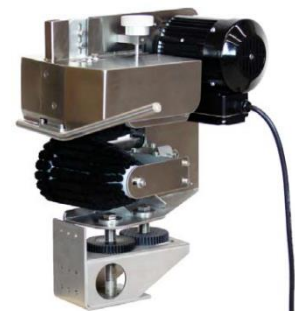
Bag Tensioner TYPE1082L8 Can gather bag's entrance prior to close it.
